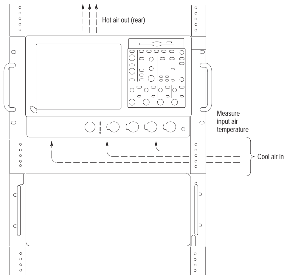
Figure 2: Instrument cooling
